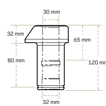
C4PX-3032-5000 Loose-fit sleeve to suit Sandvik miner-bolter, oversize head.
