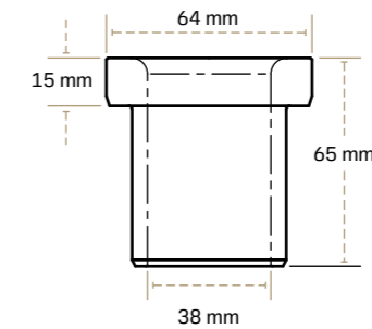
C4BB-3815-4800 Press-fit sleeve, compatible with Mitsui Miike S300 block.
