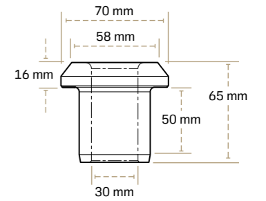
C4BB-3016-4600 Press-fit sleeve to suit Joy® J30 block.
