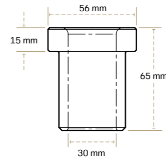
C3BB-3015-4200 Press-fit sleeve, compatible with Mitsui Miike S200 block.
