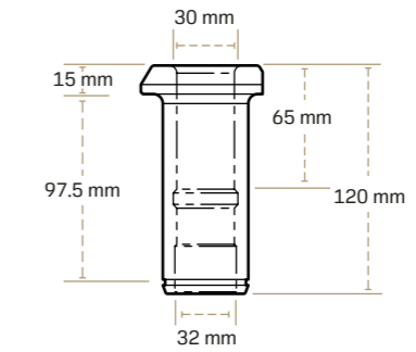
C4PK-3015-4500 Compatible with ABM20 block.
