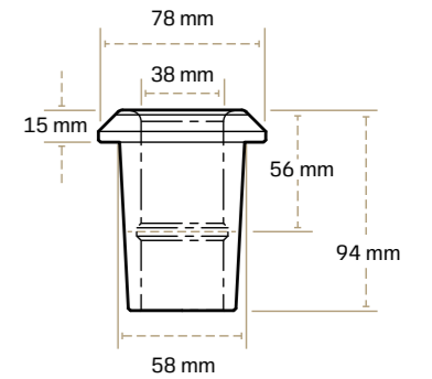
C4NS-3815-5700 Press-fit sleeve, compatible with MT720 block.
