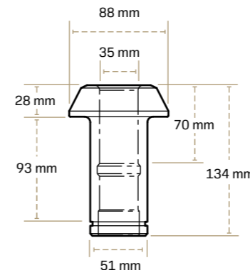
C4AA-3528-5100 Compatible with MG400 and 500 series shearers.
