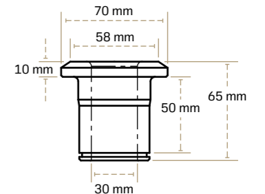
C4BU-3010-4700 Replacement sleeve for Joy® J30 block.
