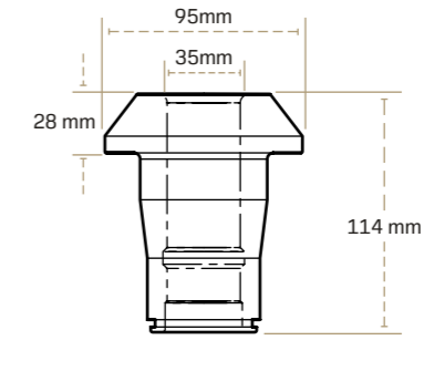
C4AK-3528-6100 Sleeve to suit J35 block.
