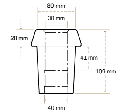
C4AS-3828-67LD Press-fit sleeve, compatible with MT720 and MT520 block.
