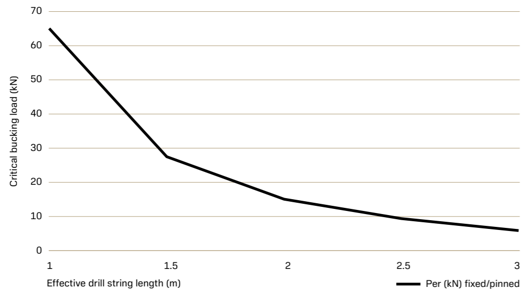
Buckling load of 22 mm hexagon drill rods
