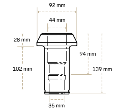
C4LA-4328-5700 Compatible with MG650 and 750 series shearers.
