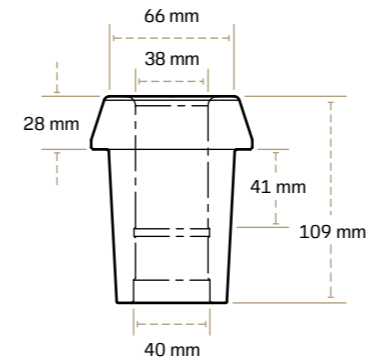
C4AS-3828-6700 Press-fit sleeve, compatible with MT720 and MT520 block.
